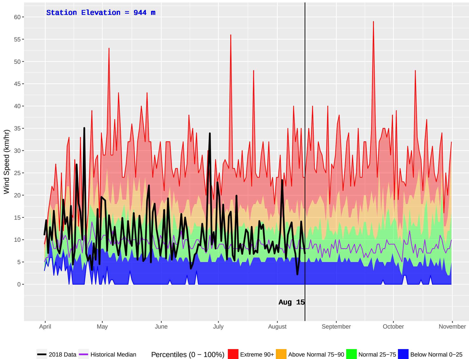
GRASSY PLAINS HUB (161) : Historical (1970–2016) and Current (2018) Daily Wind Speed
